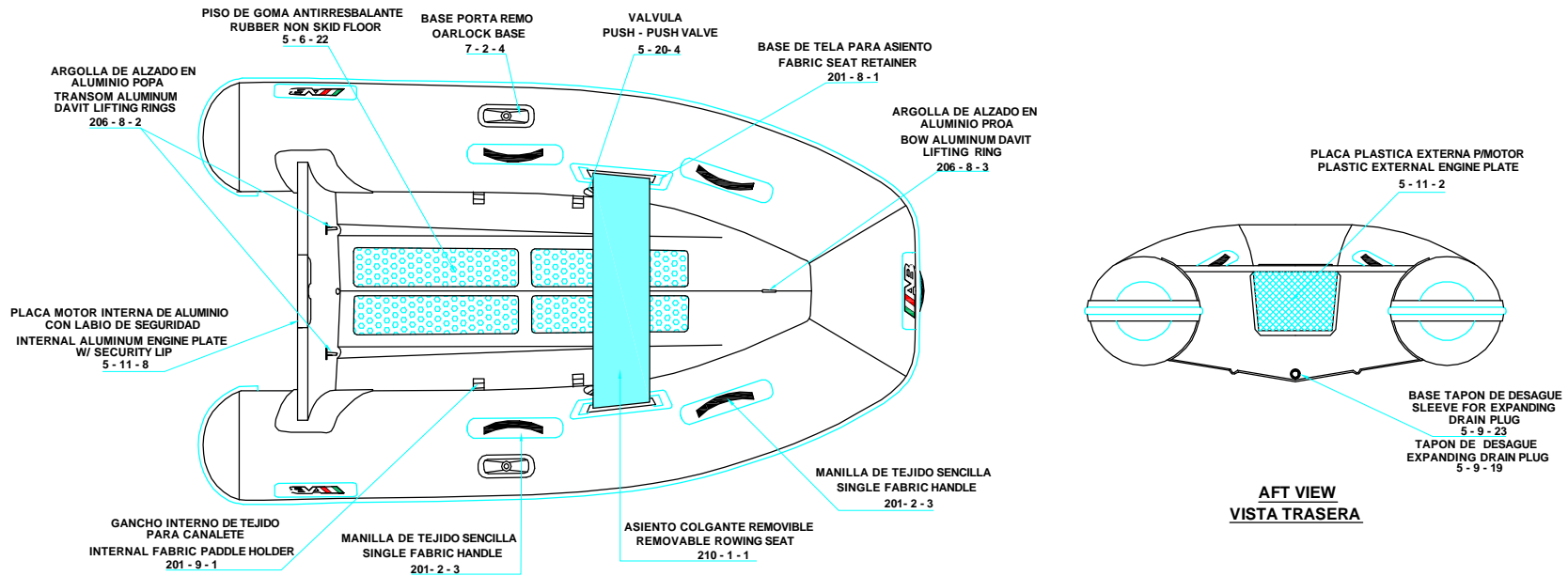
PLANT VIEW VISTA SUPERIOR
